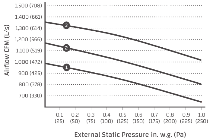
Airflows (Each Air Stream)
